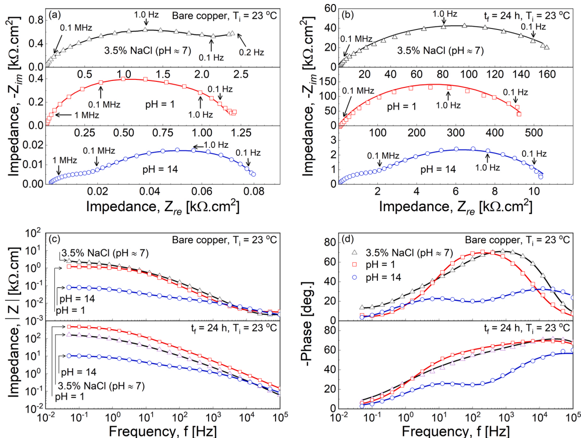
Fig. 5. EIS data curves showing the effect of pH solution at 23 °C: Nyquist plots of (a) bare copper as reference and (b) superhydrophobic surfaces (SHS); (c) Bode plots of bare copper control sample and SHS; (d) Phase diagrams of bare copper control sample and SHS.
