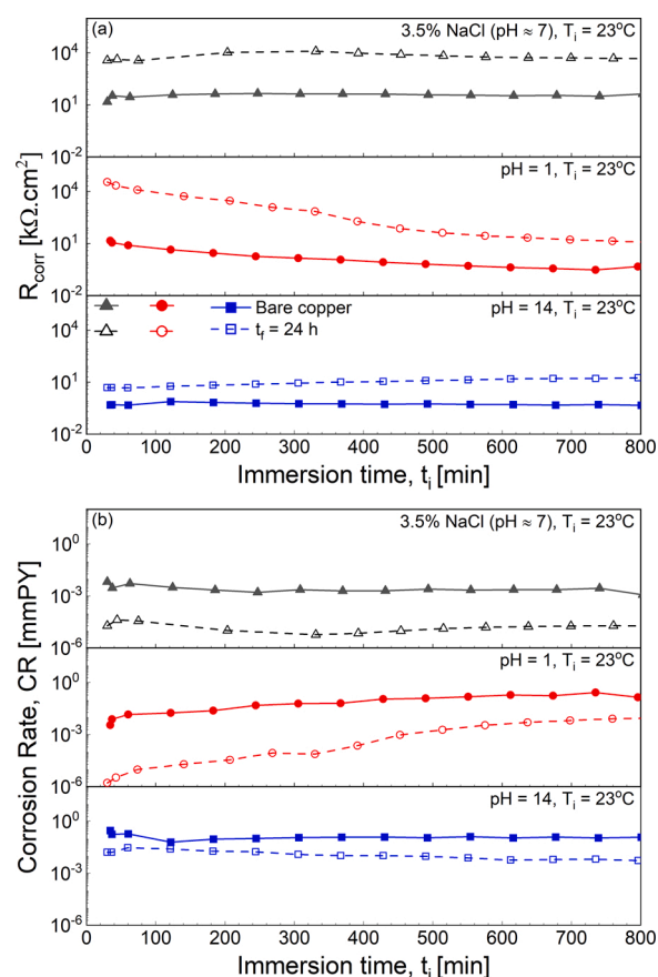
Fig. 7. Variation of (a) corrosion resistance, R_{corr} , and (b) corrosion rate, CR , with immersion time, t_i , for bare copper control sample and superhydrophobic surfaces in three different pH of the immersion solution at T_i = 23 °C.
