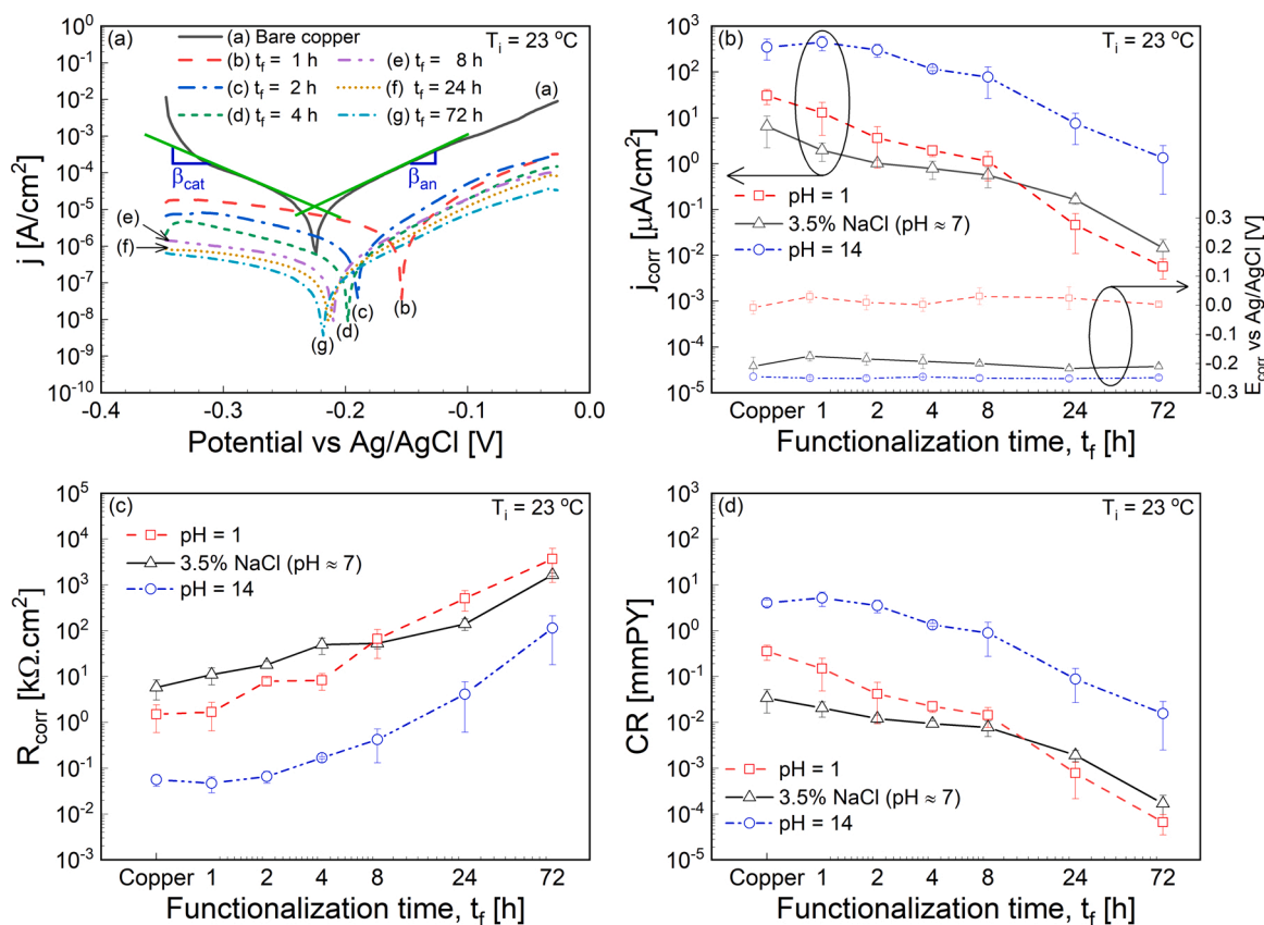
Fig. 3. (a) Tafel plots from corrosion potentiodynamic polarization (PDP) test in 3.5 % NaCl ( pH \approx 7 ) solution at 23^\circ\text{C} . Variation of corrosion parameters—(b) corrosion current, j_{corr} , and corrosion potential, E_{corr} , (c) corrosion resistance, R_{corr} , and (d) corrosion rate, CR—with functionalization time, t_f , for superhydrophobic copper surfaces at 23^\circ\text{C} at different pH solutions.
