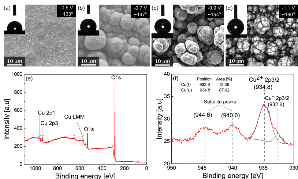
Fig. 2. (a–d) SEMs of surfaces fabricated via electrodeposition at different voltages showing progressively increasing multiscale features and corresponding hydrophobicity or superhydrophobicity; (e) XPS survey spectra and (f) XPS high resolution spectra of superhydrophobic copper surface fabricated via electrodeposition at -1.1 V and functionalized for 24 h in stearic acid.
