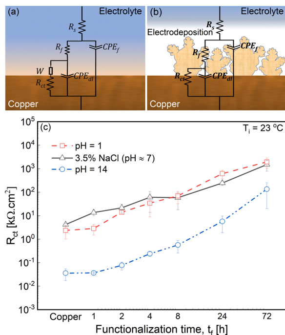
Fig. 6. Schematic of the equivalent circuit model of EIS data for (a) bare copper control sample and (b) superhydrophobic surfaces; (c) variation of the charge transfer resistance, R_{ct} , derived from the equivalent circuit model for bare copper control sample and superhydrophobic surfaces with functionalization time, t_f , in three different pH solutions.
