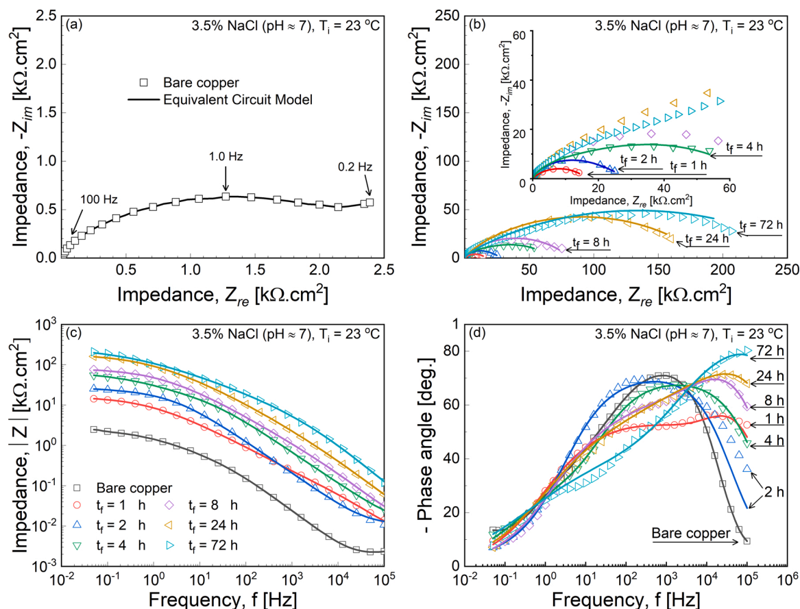
Fig. 4. EIS data curves showing the effects of functionalizing time at 23 °C in 3.5 % NaCl ( pH \approx 7 ) solution: Nyquist plots of (a) bare copper as reference, and (b) superhydrophobic surfaces (SHS); (c) Bode plots of bare copper control sample and SHS, and (d) Phase diagrams of bare copper control sample and SHS.
