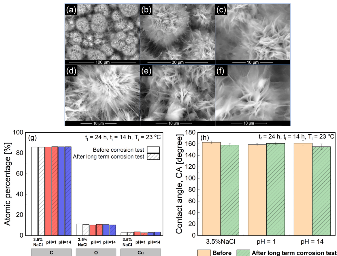
Fig. 8. SEM images of superhydrophobic surface (SHS) at three different magnifications, (a–c) before the long-term corrosion test and after long-term corrosion test in (d) 3.5 % NaCl ( pH \approx 7 ), (e) pH = 1 and (f) pH = 14 aqueous solutions; (g) summary of surface relative atomic percentage of detected elements and (h) contact angle of 10 \mu L DI-water droplet on the surfaces before and after long-term corrosion test in different pH solutions at temperature T_i = 23 °C.
