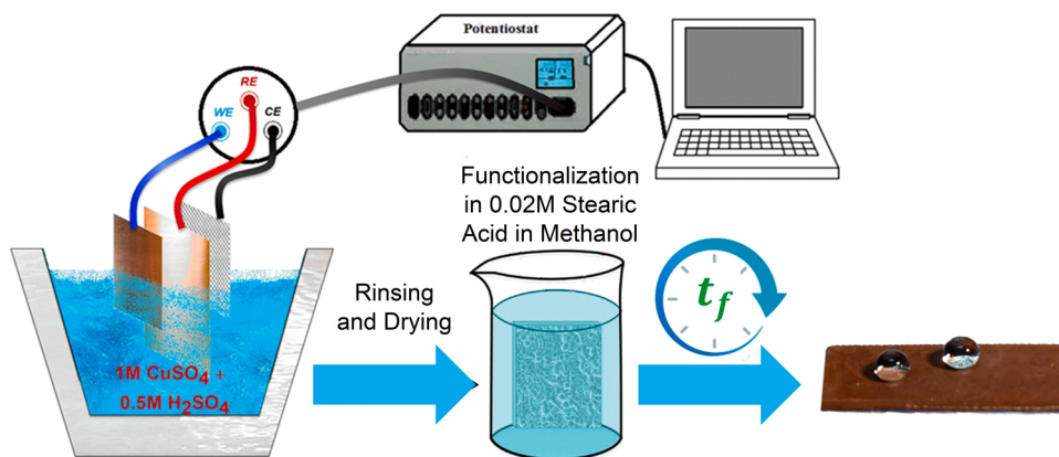
Fig. 1. Schematic of the electrodeposition setup for fabrication of superhydrophobic surfaces.
