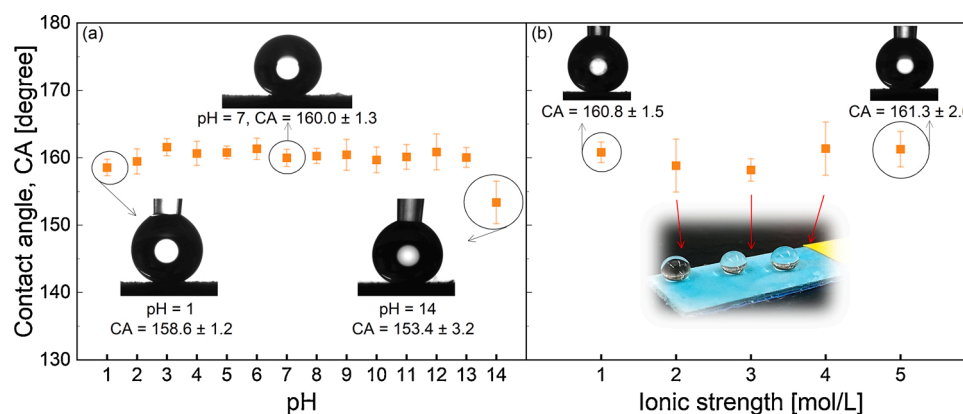
Fig. 12. Effect of (a) pH and (b) ionic strength (salinity) on the droplet contact angle for electrodeposited samples, t_f = 72 h, at room temperature. Note a 3.5 % NaCl aqueous solution corresponds to 0.6 M.
