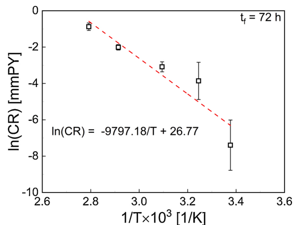
Fig. 11. Arrhenius plot of the natural logarithm of the corrosion rate in terms of the reciprocal of absolute temperature for electrodeposited superhydrophobic samples with t_f = 72 h, in 3.5 % NaCl aqueous solution.
