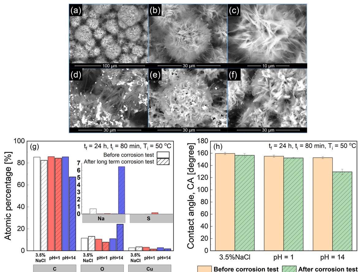
Fig. 10. SEM images of superhydrophobic surface (SHS) at three different magnifications, (a–c) before the long-term corrosion test and after long-term corrosion test in (d) 3.5 % NaCl ( pH \approx 7 ), (e) pH = 1 and (f) pH = 14 aqueous solutions; (g) summary of surface relative atomic percentage of detected elements and (h) contact angle of 10 \mu L DI-water droplet on the surfaces before and after long-term corrosion test in different pH solutions at temperature T_i = 50 °C.
